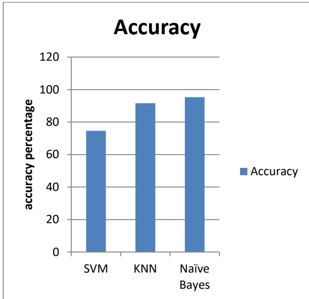
Figure 2: Accuracy Comparison
