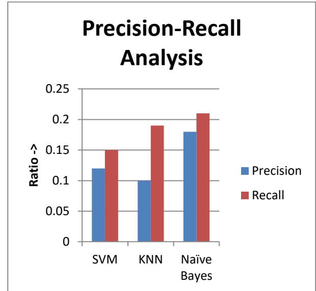
Figure 4: Precision-Recall Comparison
